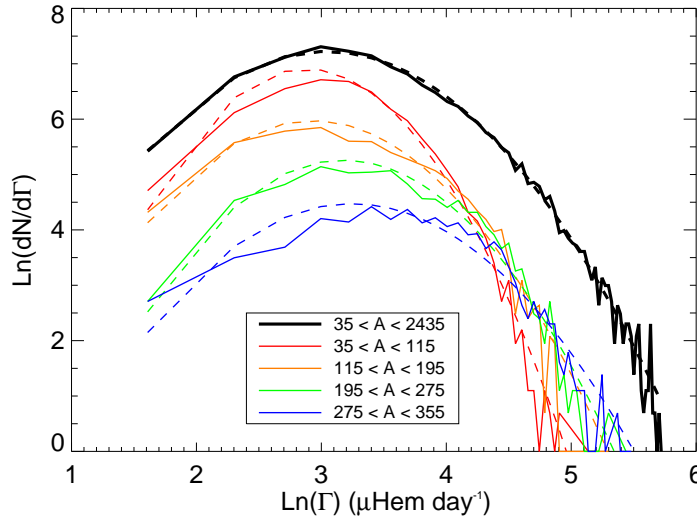
Figure 3. Distribution of decay rates for sunspot groups with areas between 35 and 2435 \mu\text{Hem} (solid black line). The distribution is very well fit by a lognormal distribution (dashed black line). The distributions of decay rates for groups binned by group area (solid colored lines) are not as well fit with lognormal distributions (dashed colored lines).
