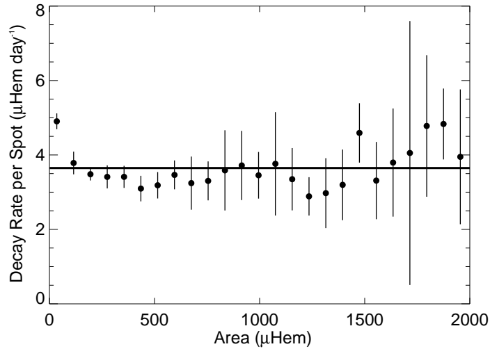
Figure 5. The ratio of the mean decay rate to the mean number of sunspots (dots with error bars) as a function of the total group area. The decay rates per sunspot are a nearly constant 3.65 \mu\text{Hem day}^{-1} for groups of all sizes except the very smallest.
