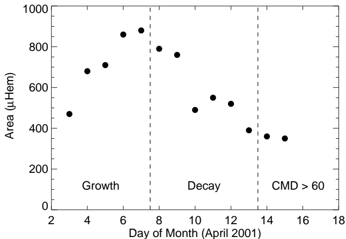
Figure 2. Sunspot group area measurements for NOAA AR 9415. The filled circles represent the daily measurements of the sunspot group area corrected for projection effects. The vertical dashed lines set off the different segments (growth, decay, and CMD > 60^\circ ) of the active region history. Our selection criteria yield two measurements of the decay rate for this sunspot group at two different values of its area.
