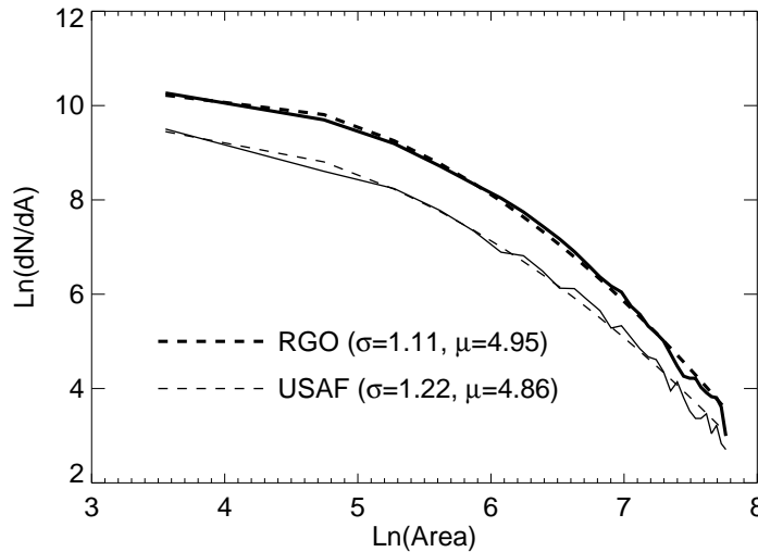
Figure 1. Sunspot group area size distributions for data from the Royal Greenwich Observatory (RGO - thick lines) and the U.S. Air Force (USAF - thin lines). The distributions are well fit with similar lognormal distributions (dashed lines — parabolic in log-log plots) but with a slightly wider distribution for the USAF data.
