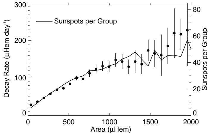
Figure 4. The decay rate of sunspot group area (dots with error bars) as a function of area itself. The decay rates increase linearly with area up to areas of about 1000 \mu\text{Hem} . The largest groups ( > 1000 \mu\text{Hem} ) have decay rates that fall somewhat below this linear relationship. The solid line shows the average number of sunspots per group as a function of area on the scale given on the right. The similarity in behavior for these two quantities suggests a constant decay rate for each individual sunspot with the number of sunspots in each group adding to the decay rate for the group itself.
