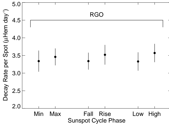
Figure 7. The mean decay rate per sunspot (dots with error bars) for different phases of the sunspot cycle and for high and low latitude groups. The higher decay rates for high latitude groups may be the source of the cycle phase and cycle-to-cycle variations in decay rate.
