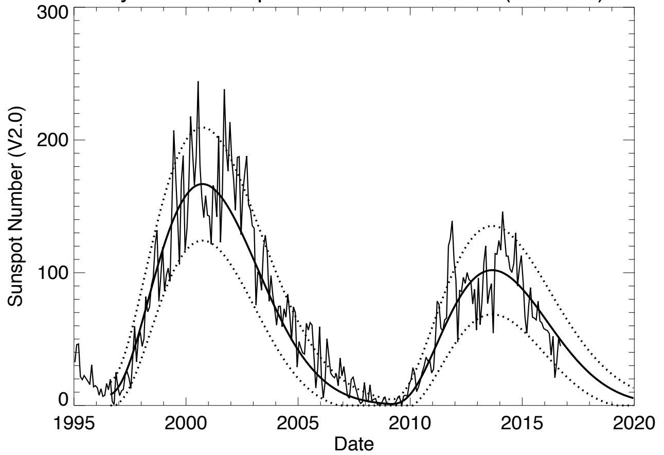
Cycle 24 Sunspot Number Prediction (2016/10)
